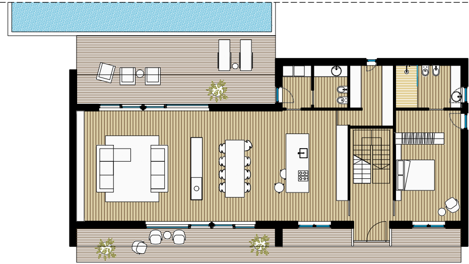
piano terra / ground floor
